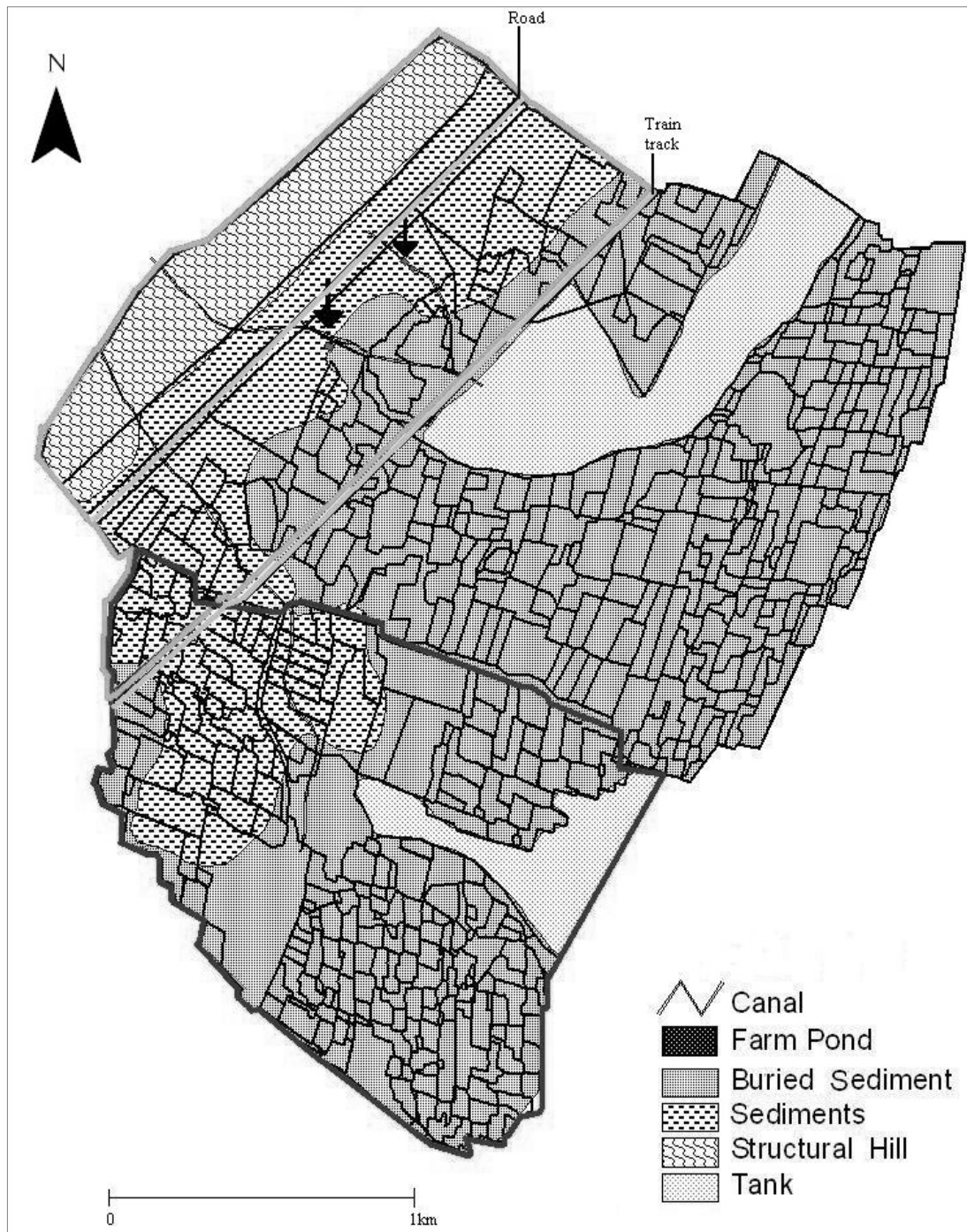
Figure 5 Arapedu watershed from geological map, approximate scale. The marked area in the southern part of the map is the area for which local authorities have kept records. Within the marked area in the western part the wells in the well inventory are located. Farm ponds are marked with arrows.
