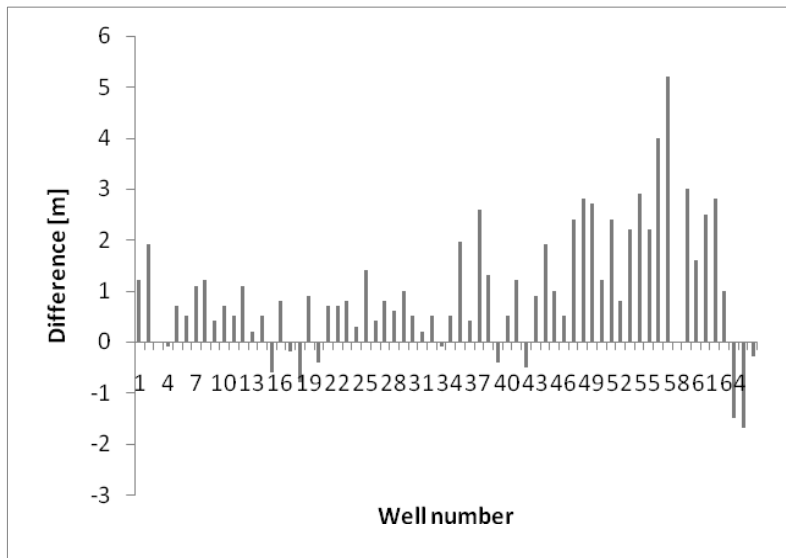
Figure 14 Difference in water level of the wells between August 2007 and August 2008. A positive value means higher water level in 2008 and a negative value means lower. Each bar represents one well.
